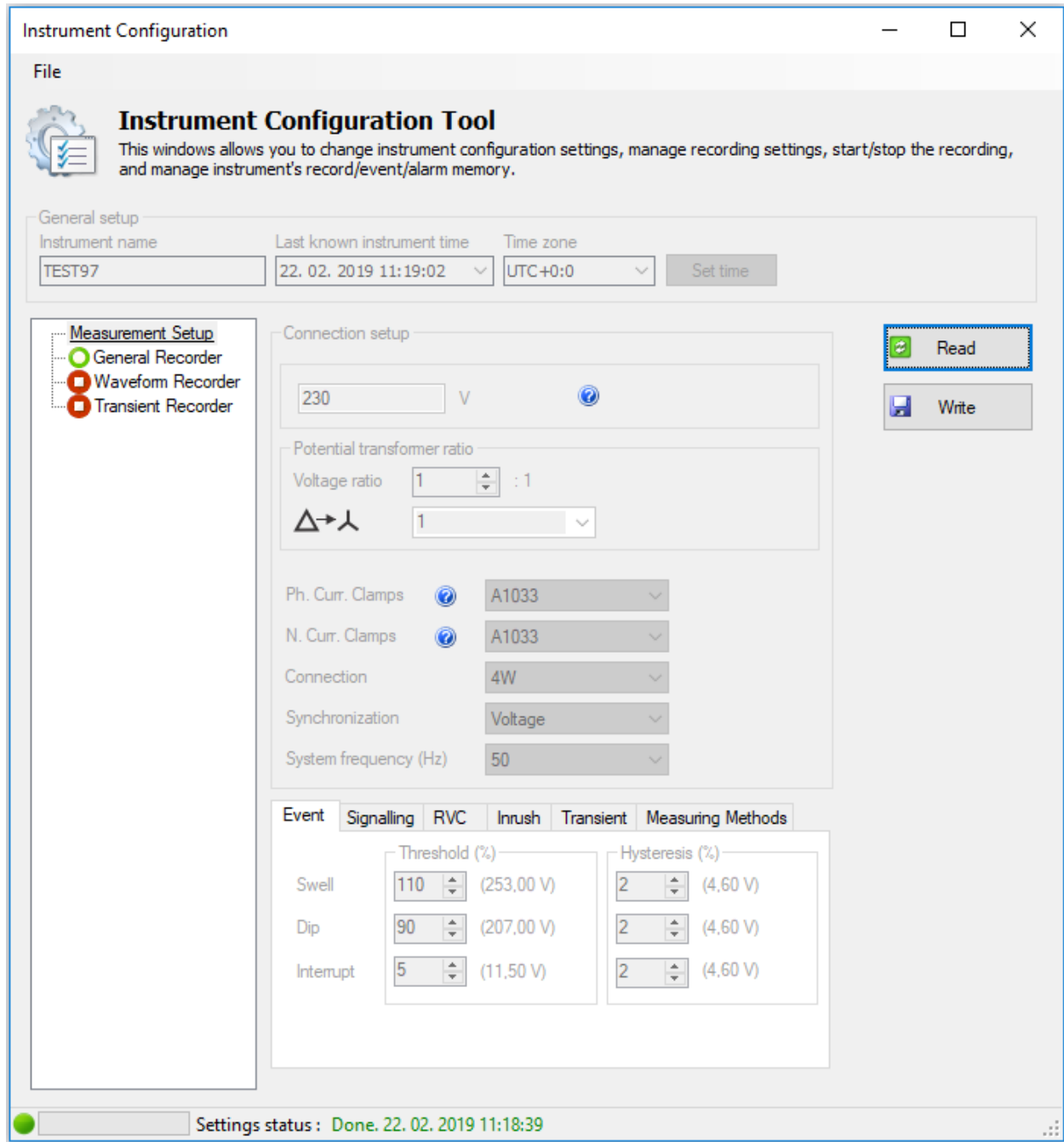
Figure 44: Remote Instrument Configuration form
