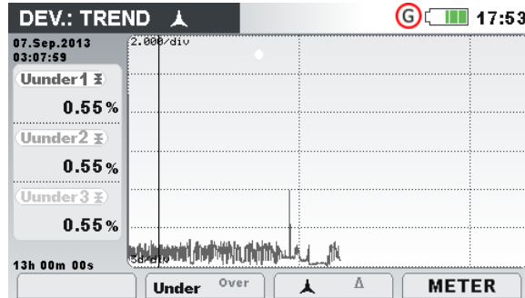
Figure 49: Under-deviation and over-deviation TREND screen
