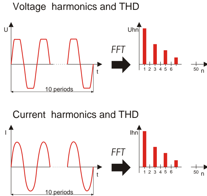
Figure 143: Current and voltage harmonics
