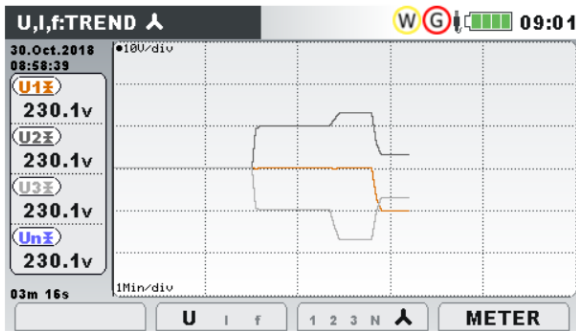
Figure 21: Voltage trend (all voltages)
