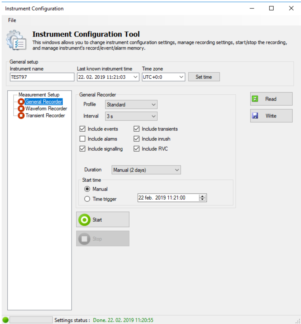
Figure 45: Remote Recorder configuration
