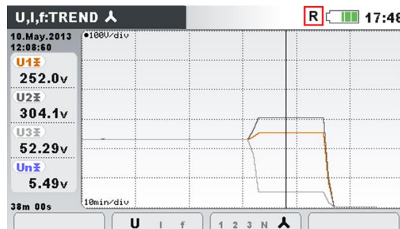
Figure 71: Viewing recorder U,I,f TREND data
