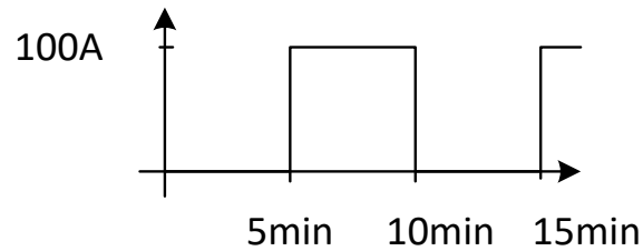
Figure 152: Avg vs. Avgon, switching load current
