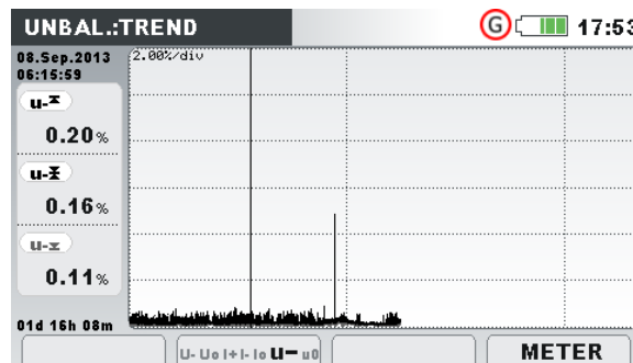
Figure 45: Symmetry trend screen
