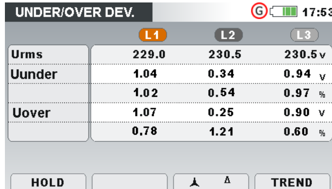
Figure 48: Under deviation and over deviation table screen
