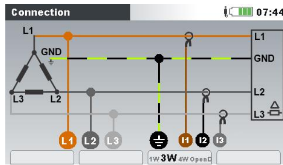
Figure 5: Choosing 3-phase 3-wire system on instrument
