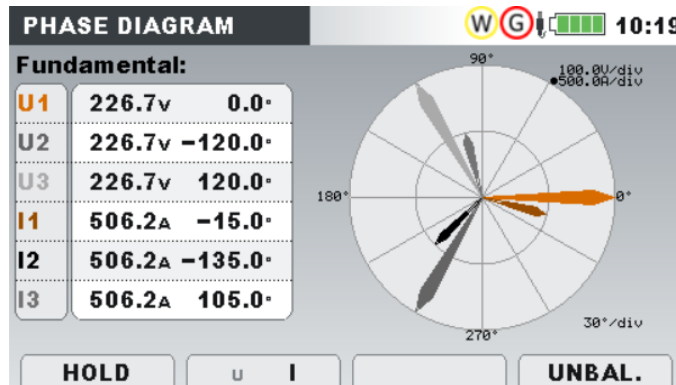
Figure 43: Phase diagram screen
