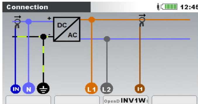
Figure 13: Choosing single- phase Inverter system on instrument
