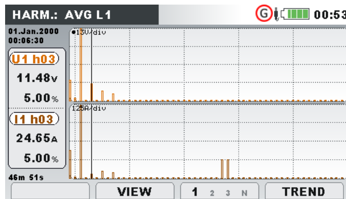
Figure 39: Harmonics average histogram screen
