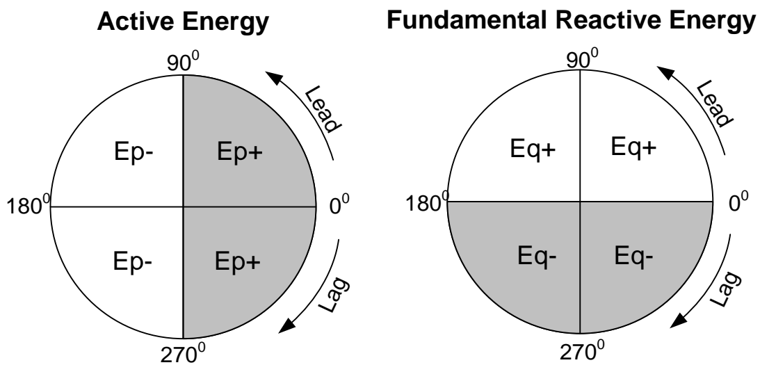
Figure 141: Energy counters and quadrant relationship
