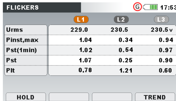
Figure 41: Flickers table screen
