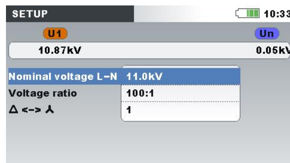
Figure 17: Voltage ratio for 11 kV / 110 kV transformer example
