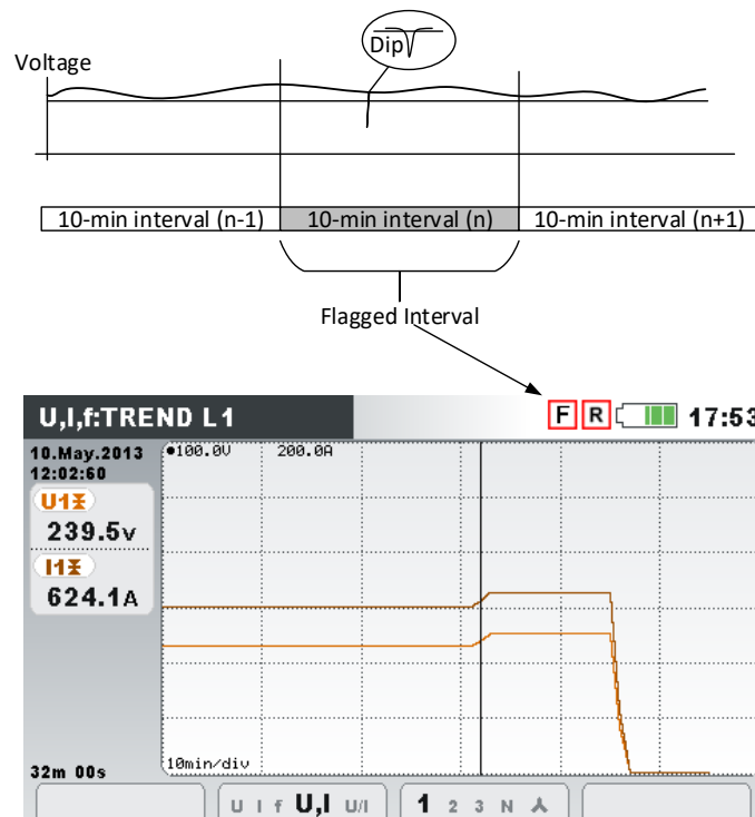
Figure 154: Flagging data indicate that aggregated value might be unreliable
