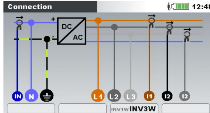
Figure 15: Choosing three- phase Inverter system on instrument
