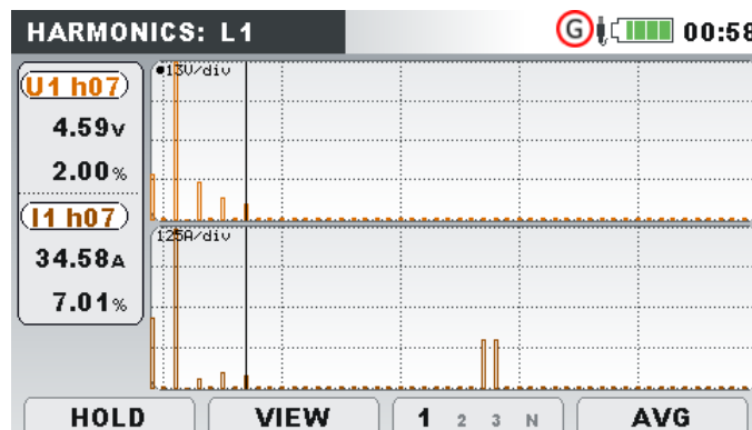
Figure 38: Harmonics histogram screen
