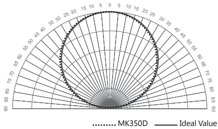
Figure 1 : Cosine Correction
